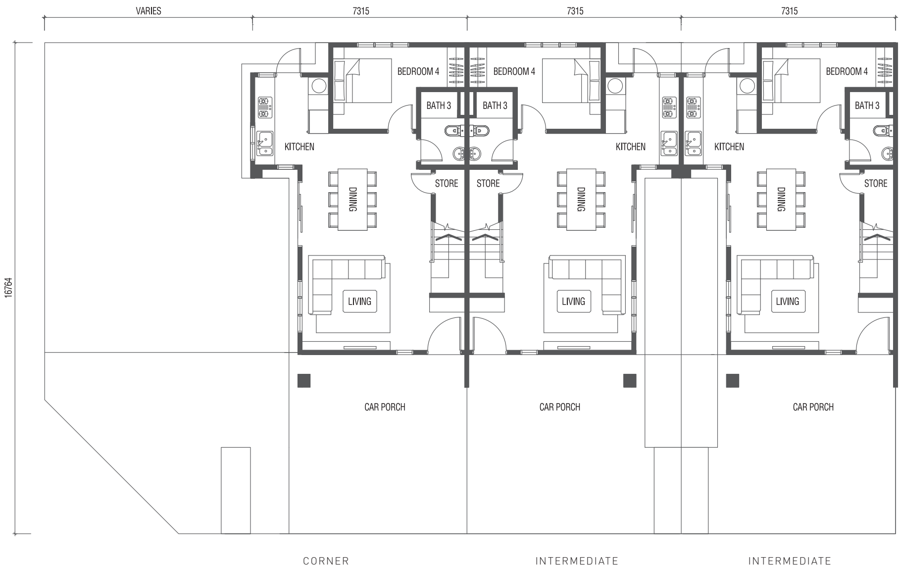
GROUND FLOOR
