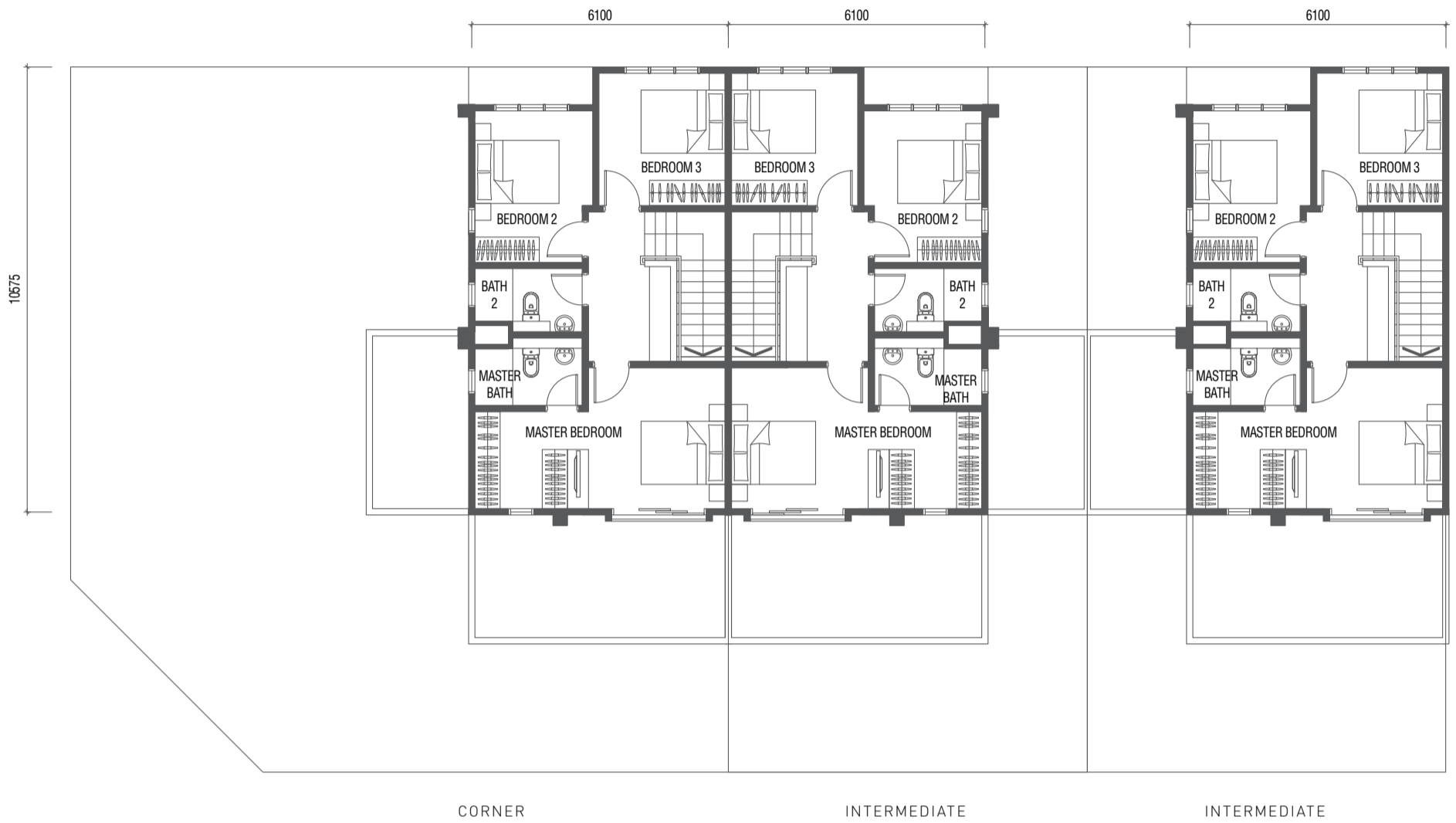
FIRST FLOOR
