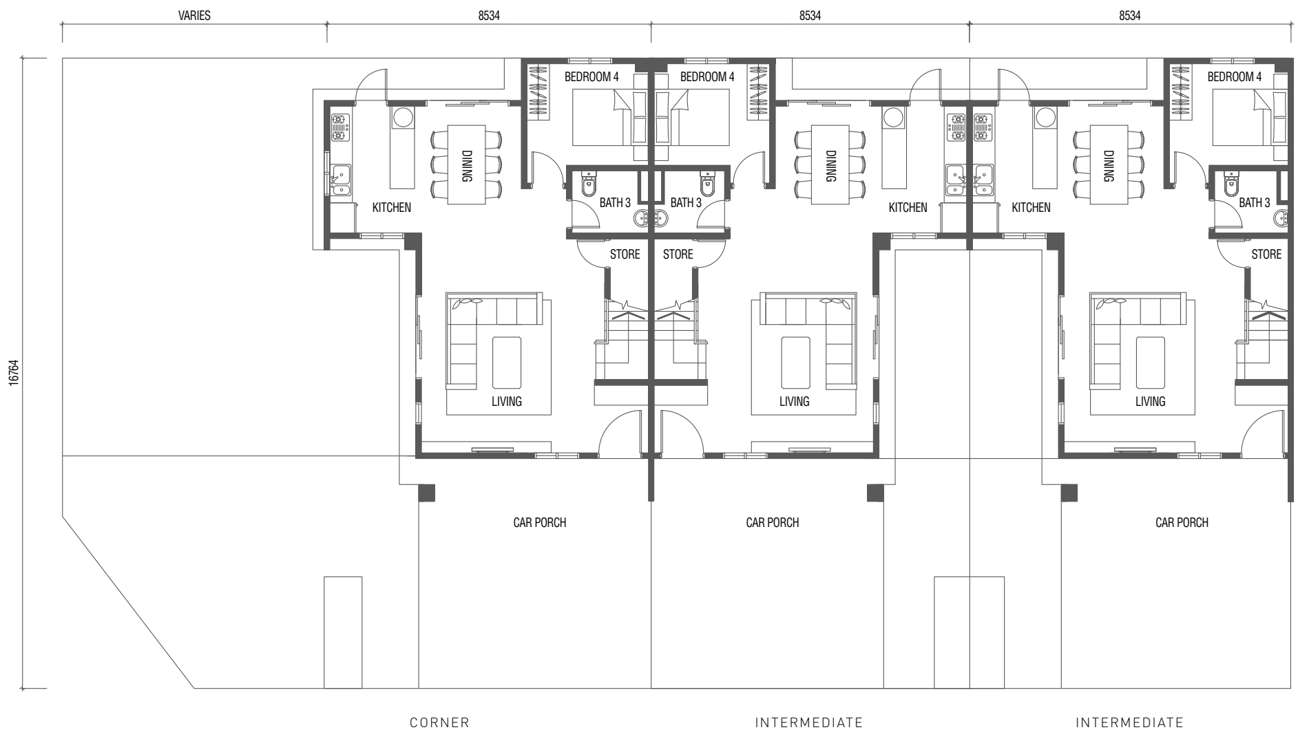
GROUND FLOOR
