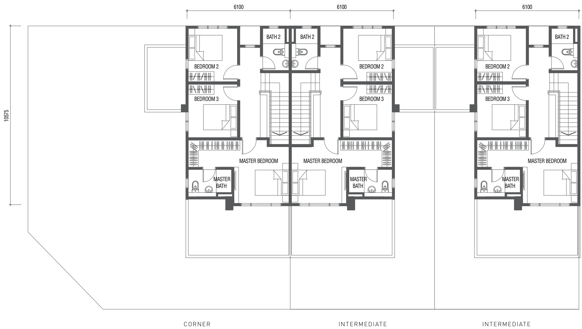
FIRST FLOOR
