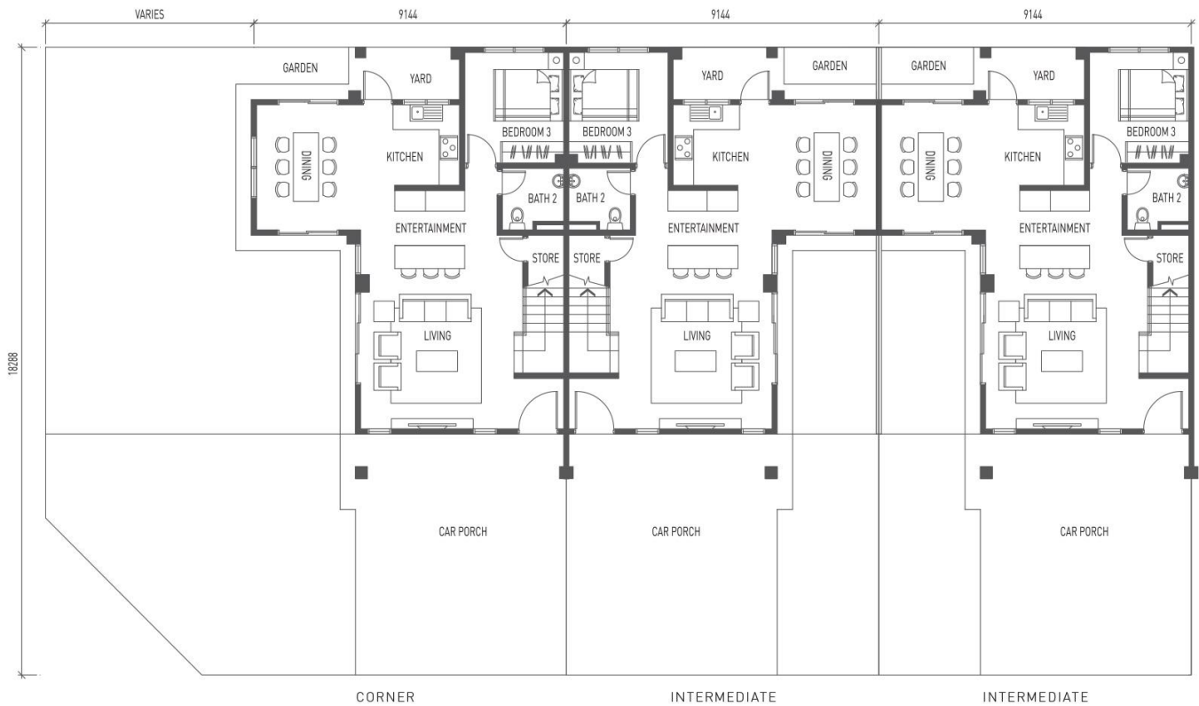
GROUND FLOOR
