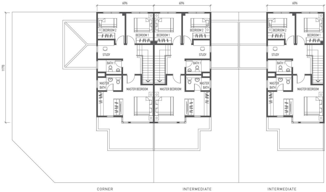
FIRST FLOOR
