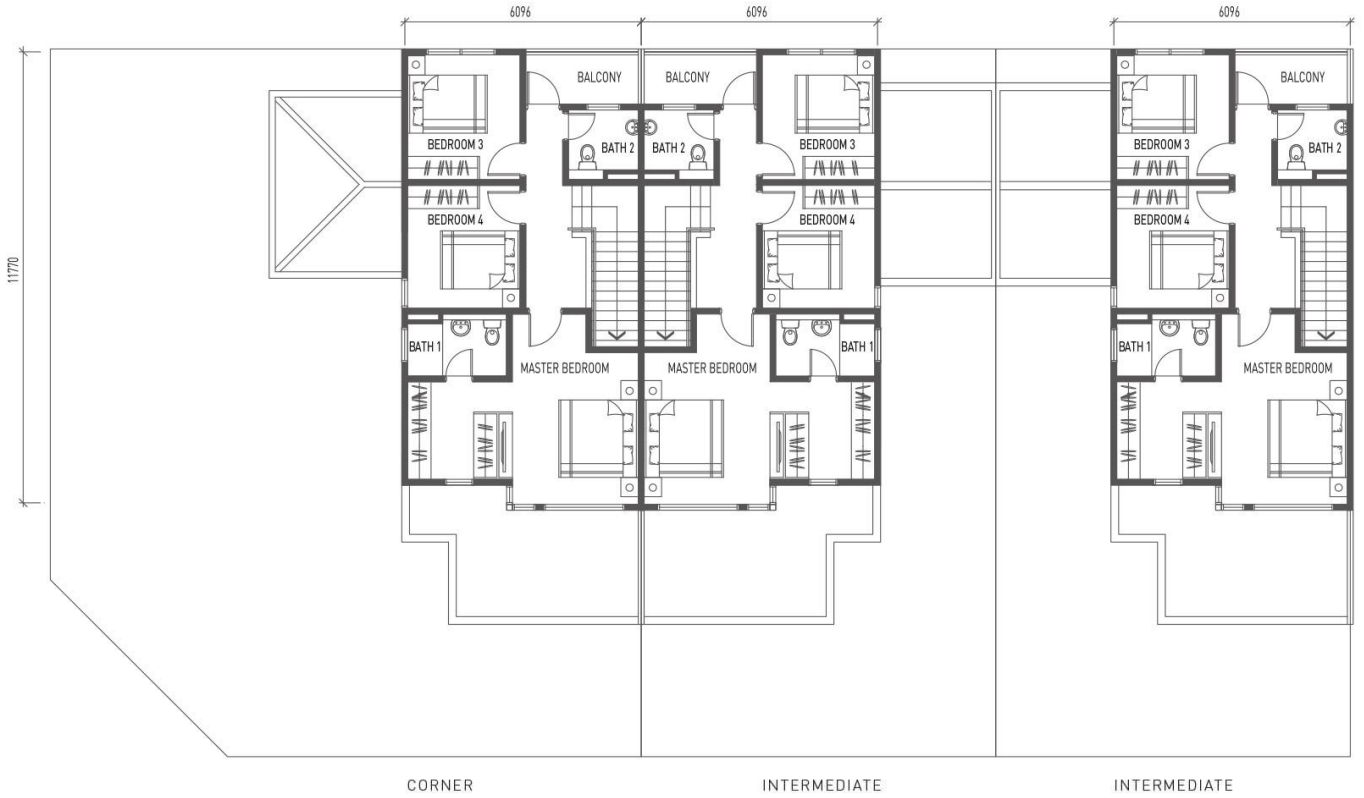
FIRST FLOOR
