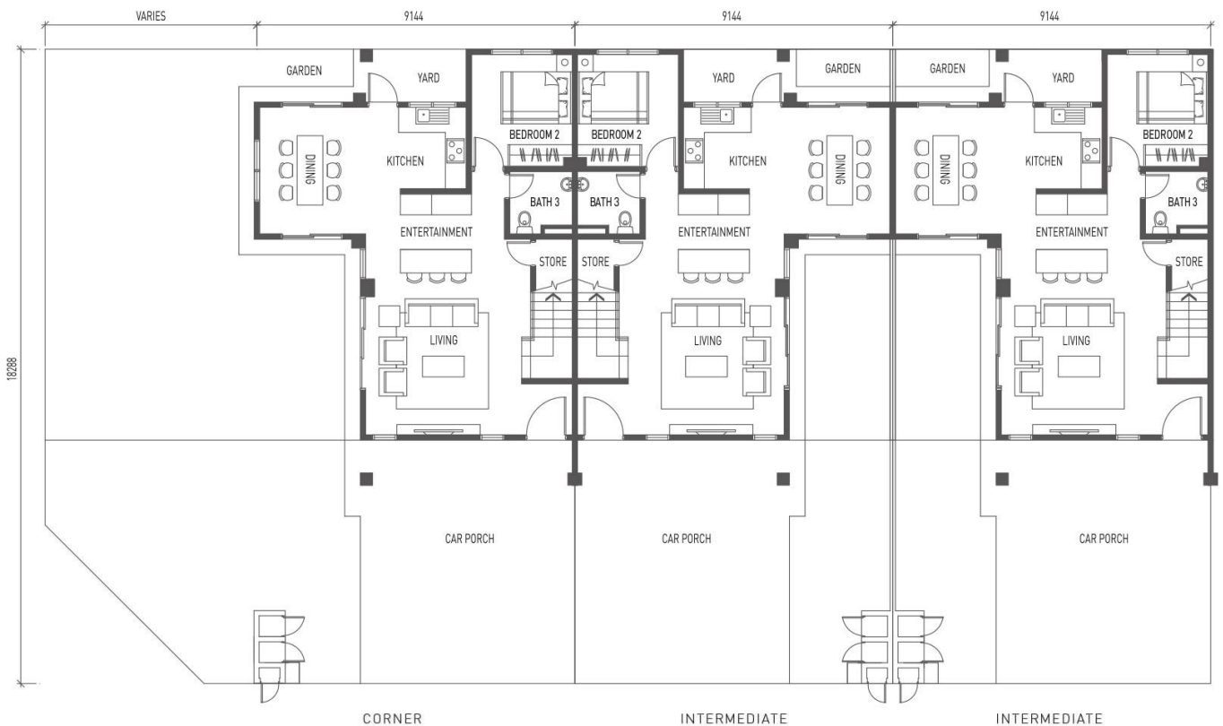
GROUND FLOOR
